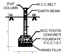
FOUNDATION DETAILS
