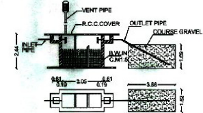
SEPTIC TANK & DISPERSION TRENCH DETAILS
