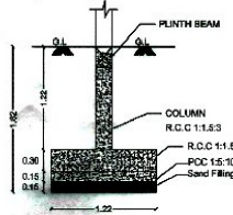
FOUNDATION DETAILS-A
