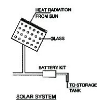
SOLAR SYSTEM
