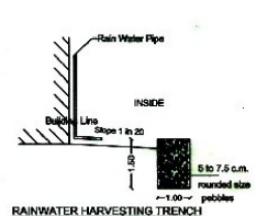
RAINWATER HARVESTING TRENCH
