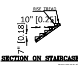
SECTION ON STAIRCASE
