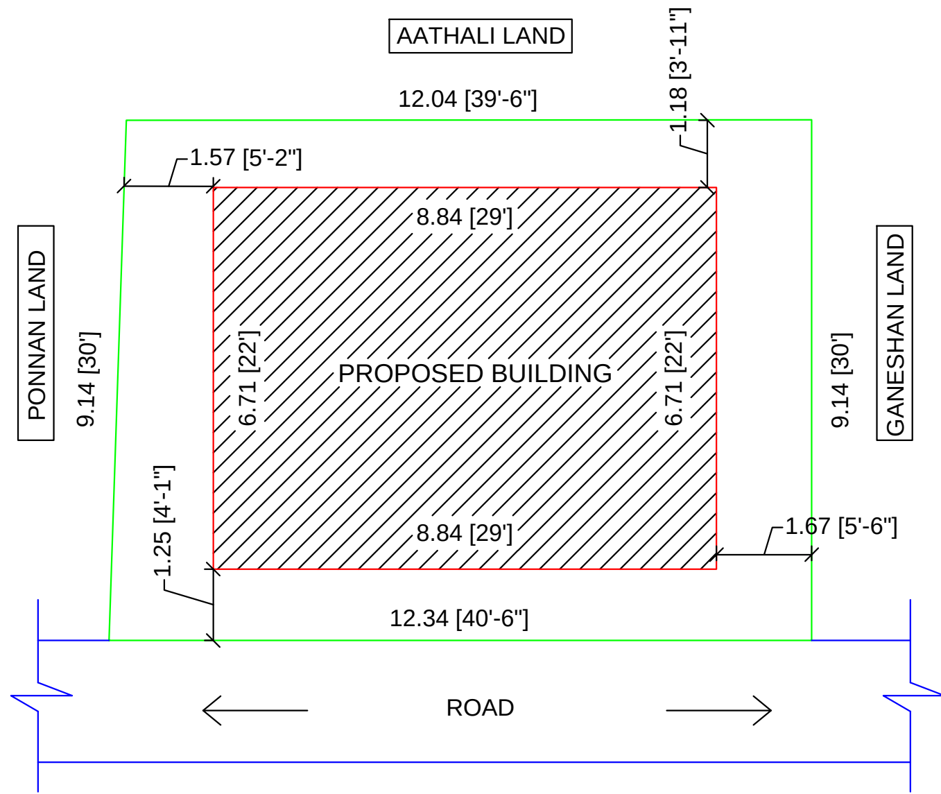
SITE PLAN
