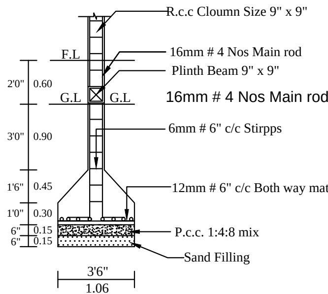
COLUMN DETIAL
