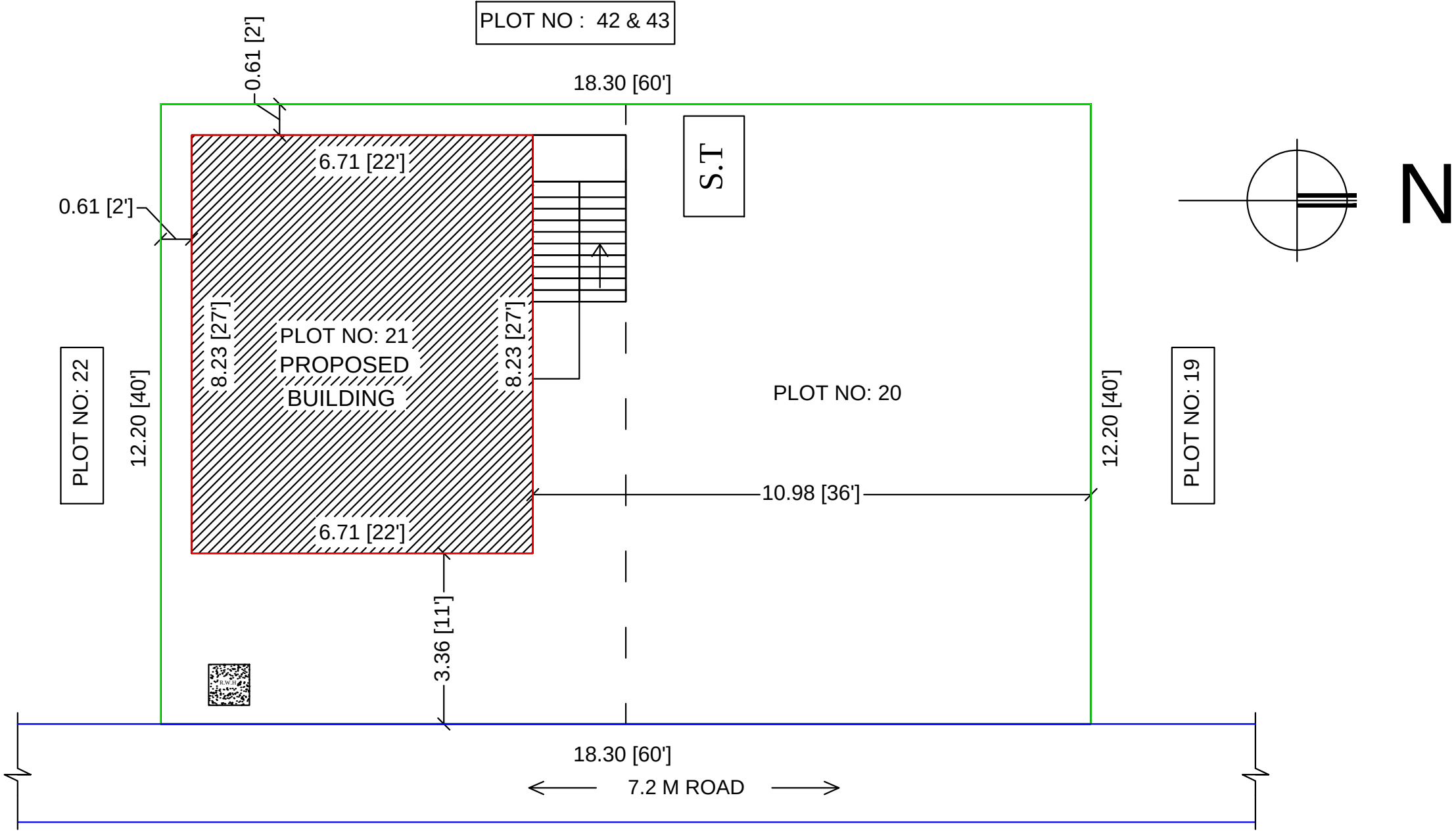
SITE PLAN
