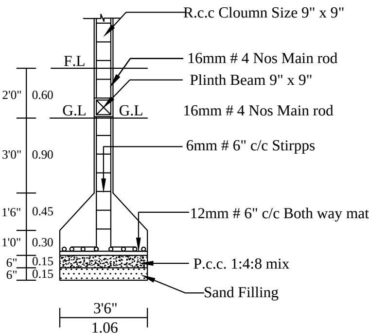
COLUMN DETIAL
