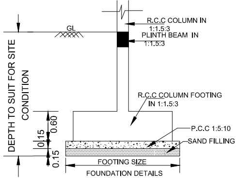
FOUNDATION DETAILS NOT TO SCALE
