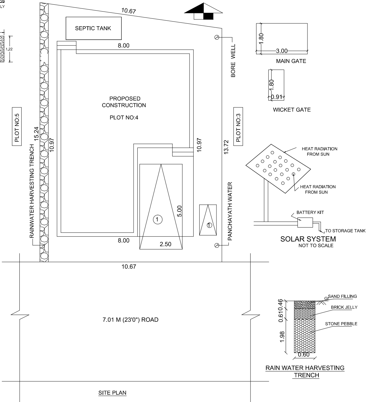
DETAIL
