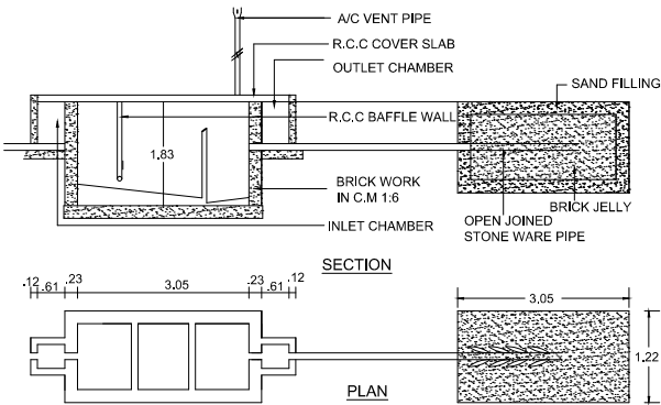
PLAN DETAILS OF SEPTIC TANK AND DISPERSION TRENCH
