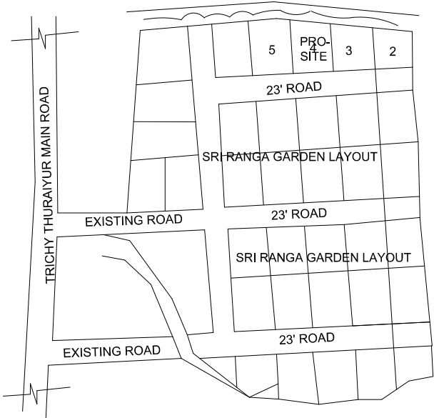
TOPO PLAN SCALE:1:1000
