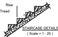
STAIRCASE DETAILS ( Scale = 1 : 25 )
