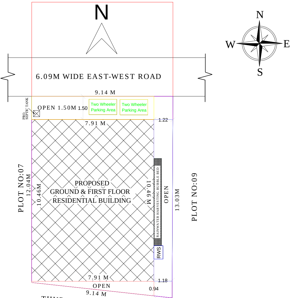
SITE PLAN (SCALE 1:1)
