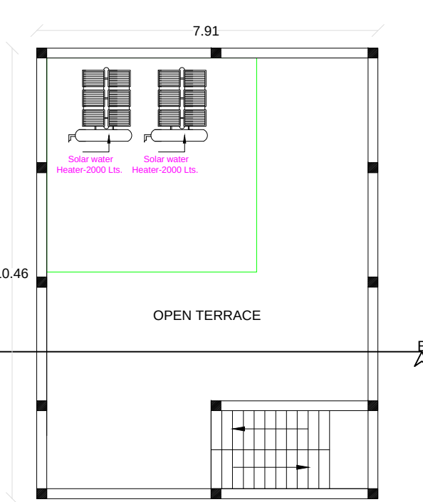
AT OPEN TERRACE
