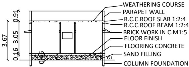
SECTION- SS
