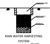
RAIN WATER HARVESTING SYSTEM (NOT TO SCALE)
