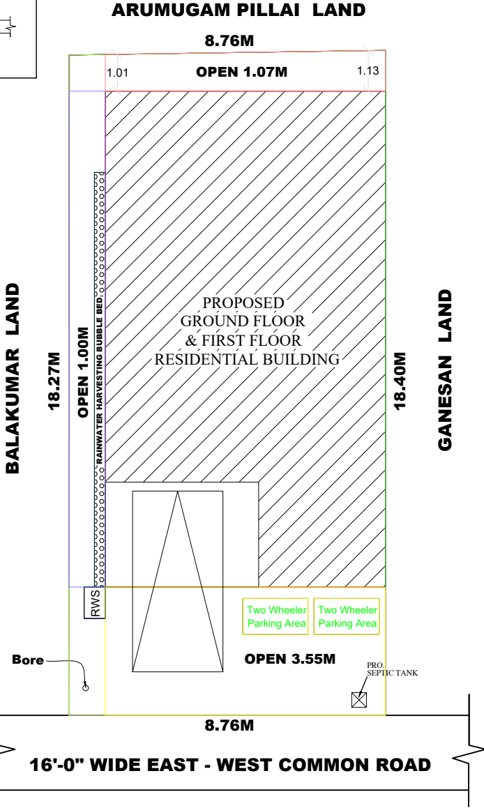
SITE PLAN (SCALE 1:1)
