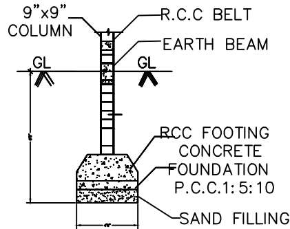
FOUNDATION DETAILS
