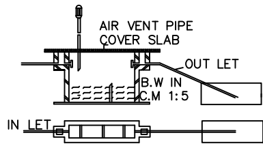
DETAILS OF SEPTIC TANK & D-TRENCE
