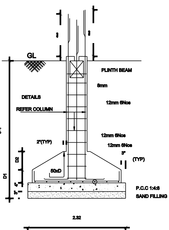
FOUNDATION DETAILS SCALE : 1:50.
