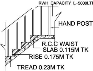
DETAILS OF STAIRCASE
