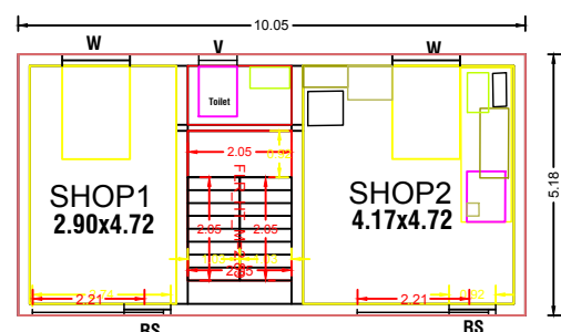
PRO.,GROUND FLOOR PLAN
