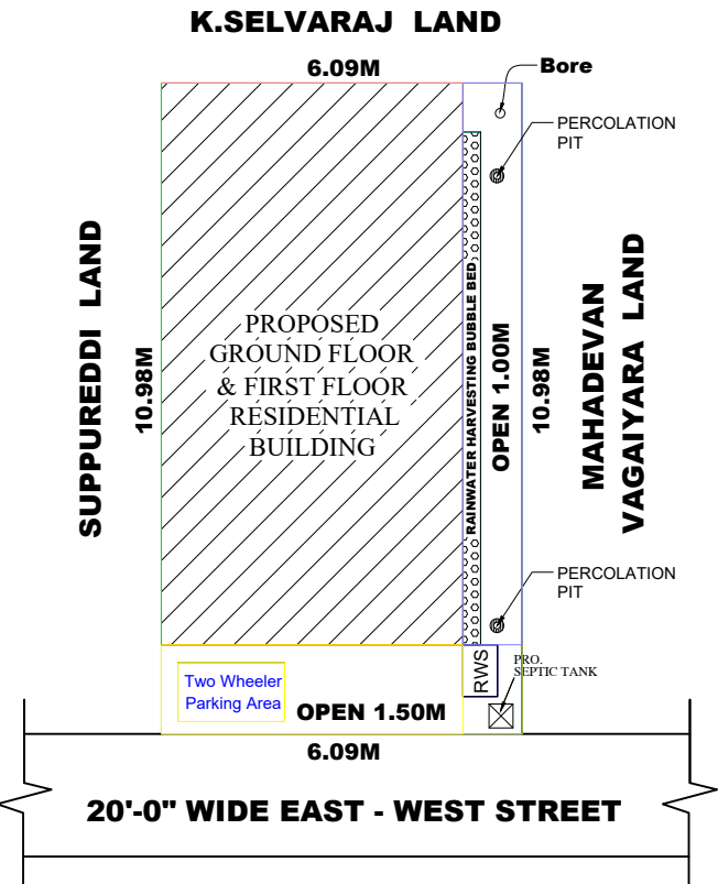
SITE PLAN (SCALE 1:1)
