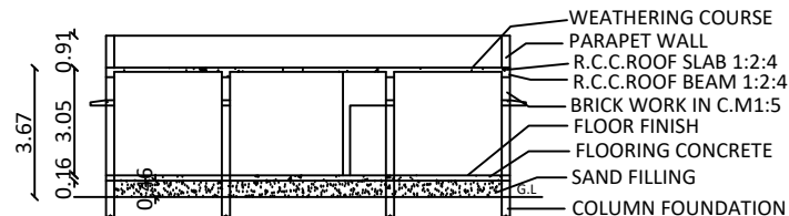
SECTION- SS
