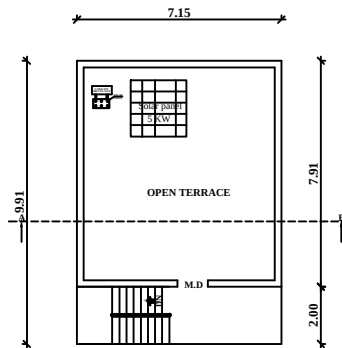
TERRACE FLOOR
