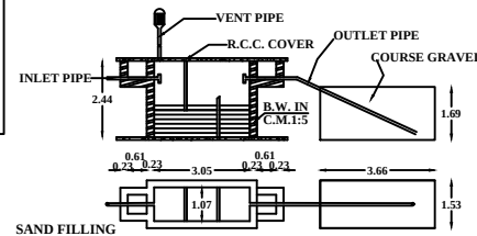
SEPTIC TANK & OF DISPERSION TRENCH DETAILS (NOT TO SCALE)
