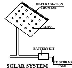
SOLAR SYSTEM (NOT TO SCALE)
