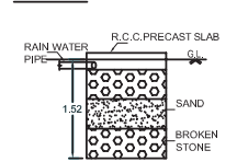
RAINWATER HARVESTING ARRANGEMENTS
