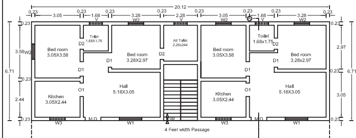
TYPICAL FIRST FLOOR & SECOND FLOOR PLAN
