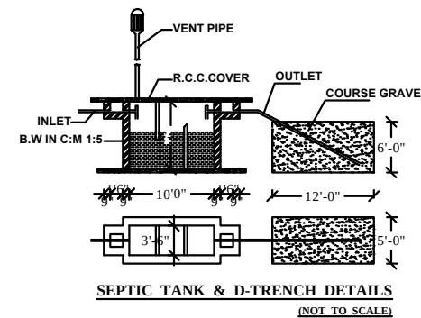
SEPTIC TANK & D-TRENCH DETAILS (NOT TO SCALE)
