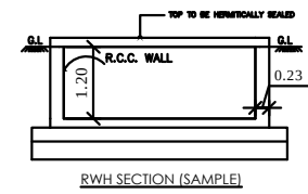
RWH_CAPACITY_L=2000LTRS
