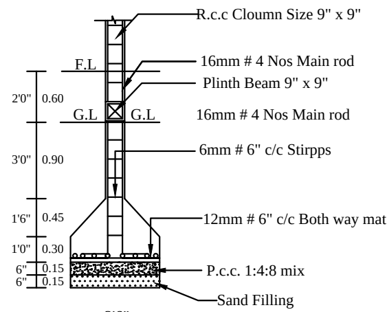
COLUMN DETIAL
