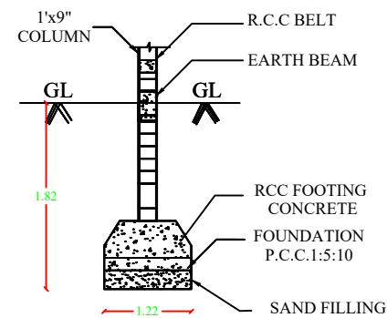
FOUNDATION DETAILS
