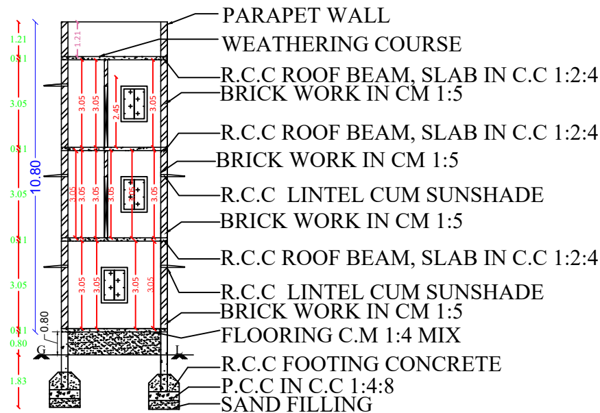
SECTION AB
