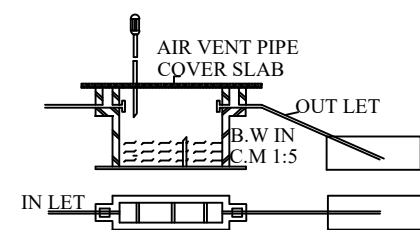
DETAILS OF SEPTIC TANK & D-TRENCE
