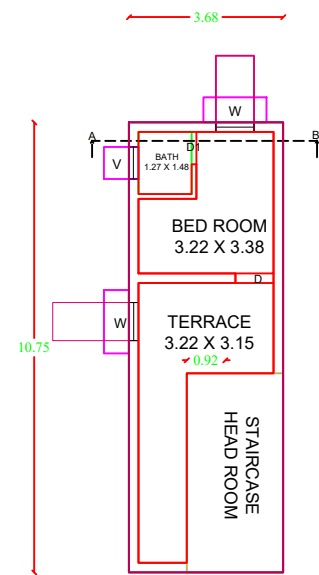
PROPOSED SECOND FLOOR PLAN
