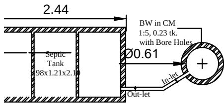
SEPTIC TANK & SOAK PIT
