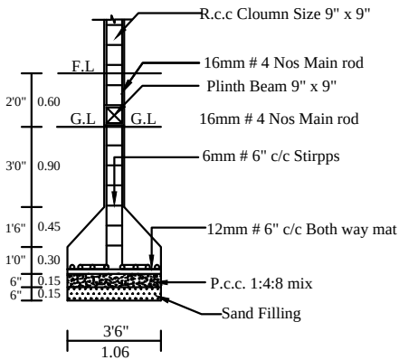
COLUMN DETIAL
