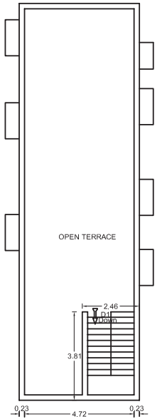
PROPOSED TERRACE FLOOR PLAN
