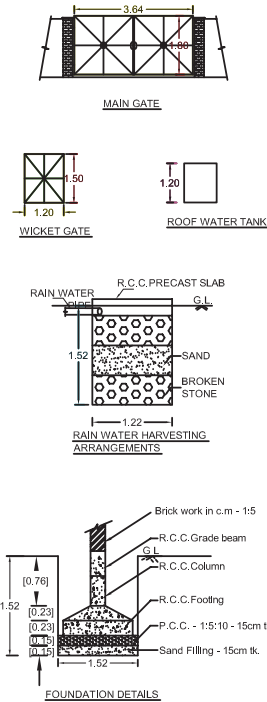
FOUNDATION DETAILS
