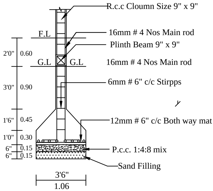
COLUMN DETIAL
