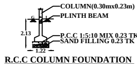
R.C.C. COLUMN FOUNDATION
