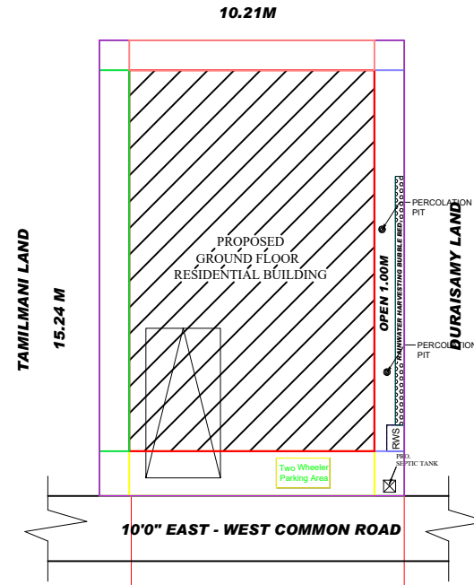
SITE PLAN (SCALE 1:1)
