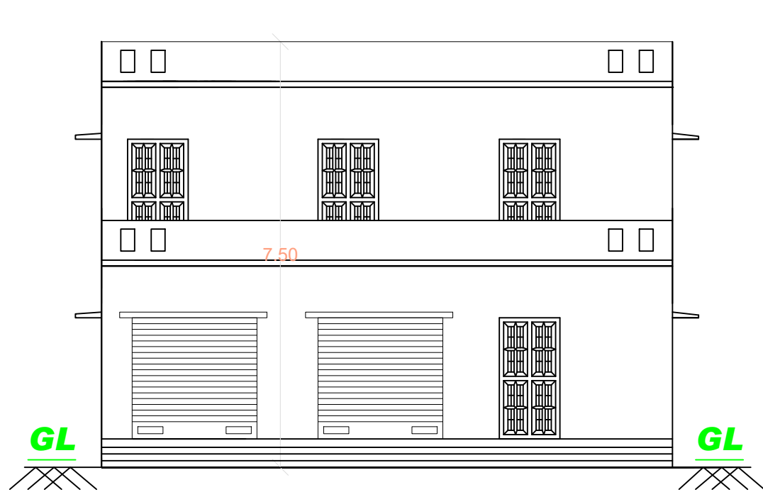
FRONT ELEVATION
