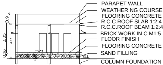
SECTION- SS
