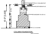
COLUMN FOUNDATION (NOT TO SCALE)
