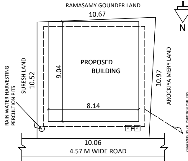
SITE PLAN
