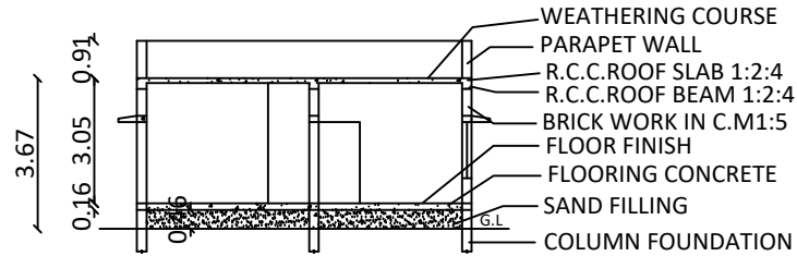
SECTION- SS
