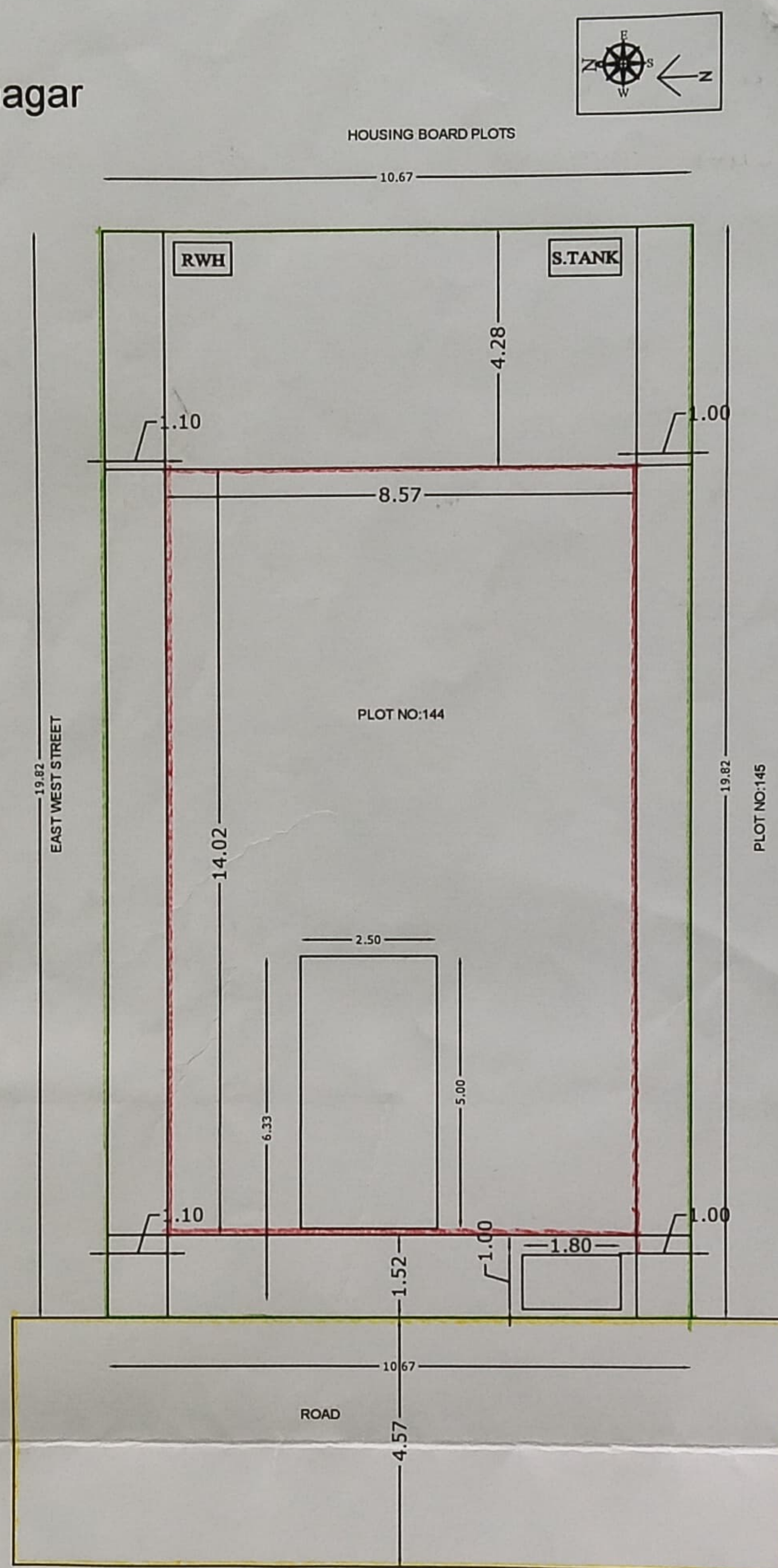
SITE PLAN
