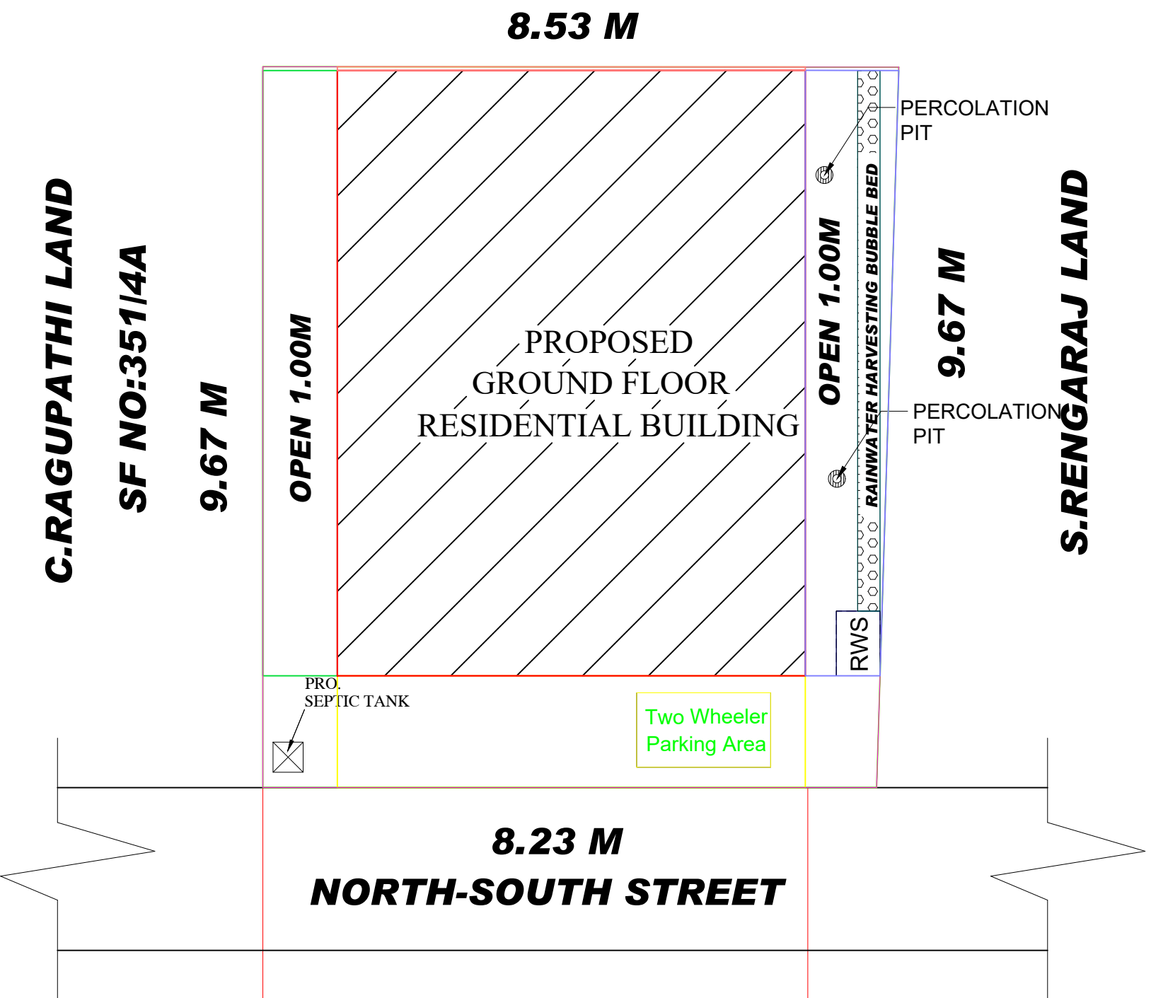
SITE PLAN (SCALE 1:1)
