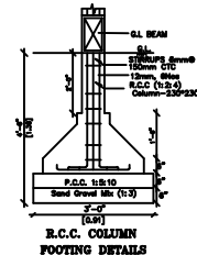
R.C.C. COLUMN FOOTING DETAILS
