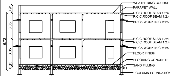
SECTION ON SS
