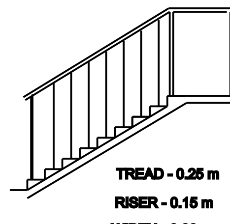
STAIRCASE DETAILS
