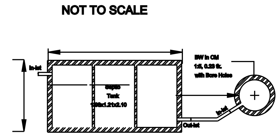
PLAN - SEPTIC TANK & SOAK PIT
