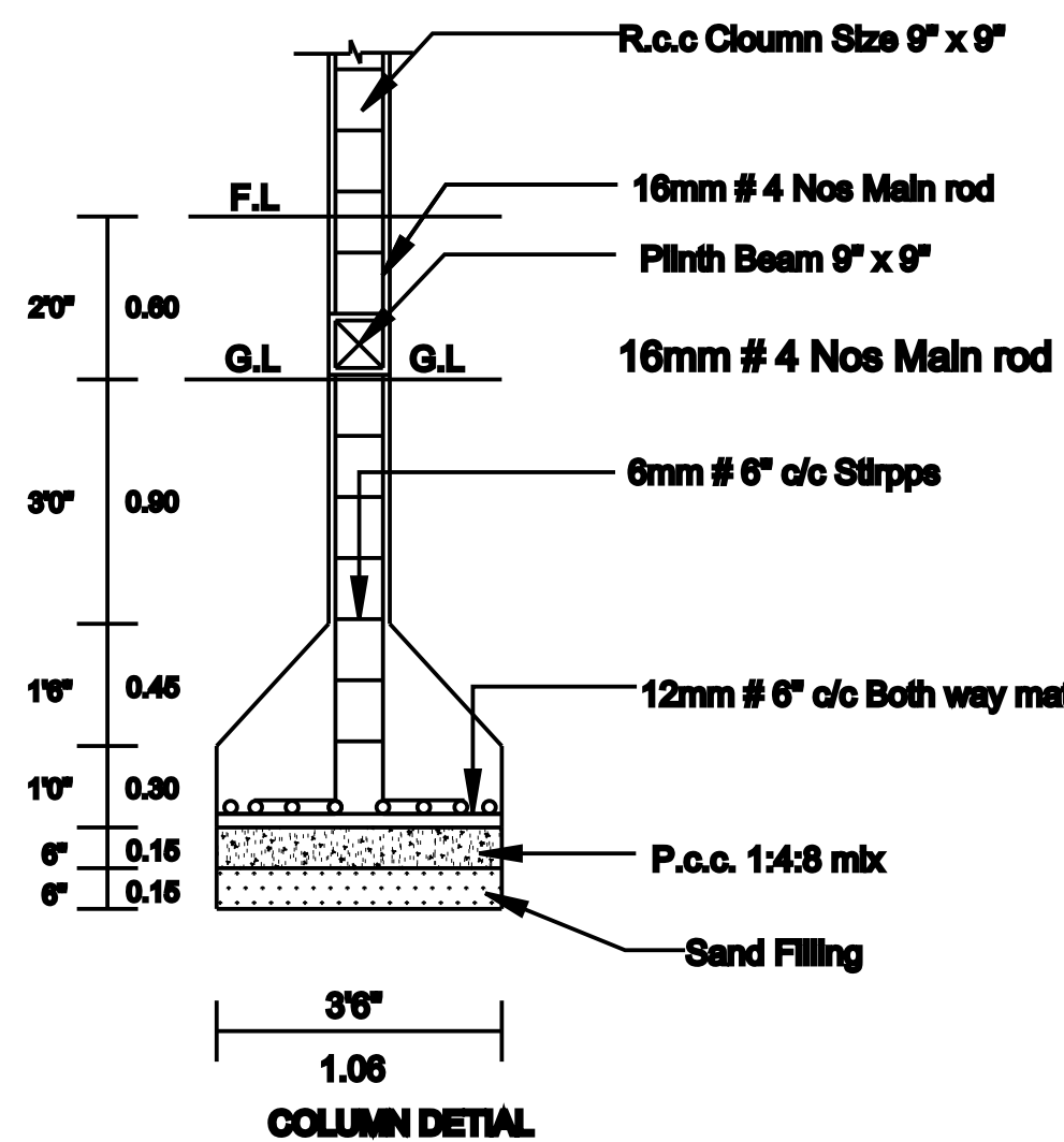
COLUMN DETAIL
