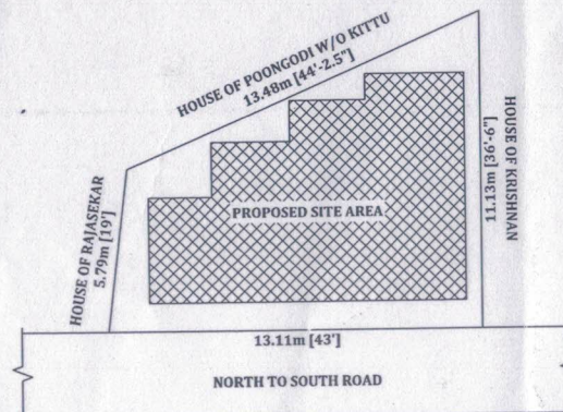
SITE PLAN [WEST FACING]
