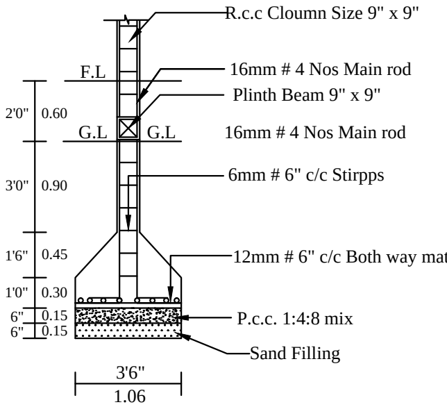
COLUMN DETIAL
