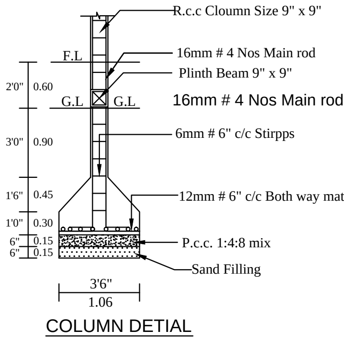
COLUMN DETIAL
