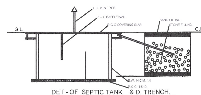
DET - OF SEPTIC TANK & D. TRENCH.
