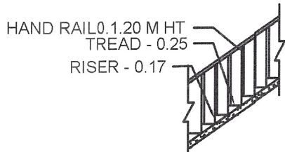
DET - OF STAIRCASE
