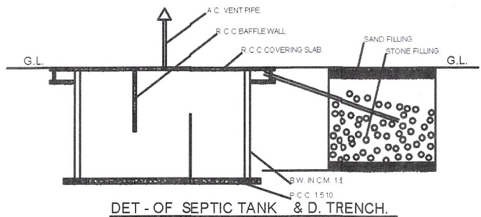
DET - OF SEPTIC TANK & D. TRENCH.
