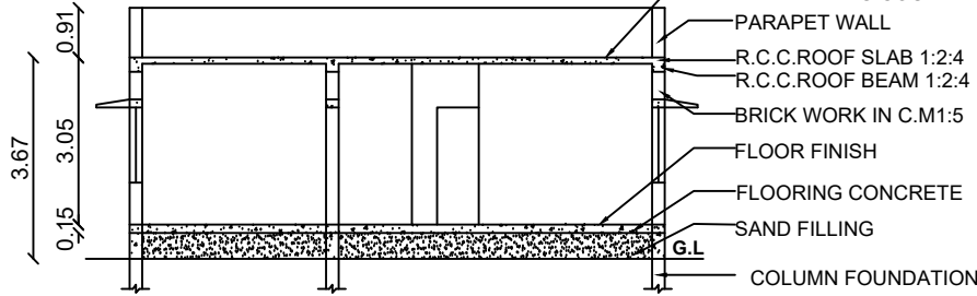
SECTION ON SS
