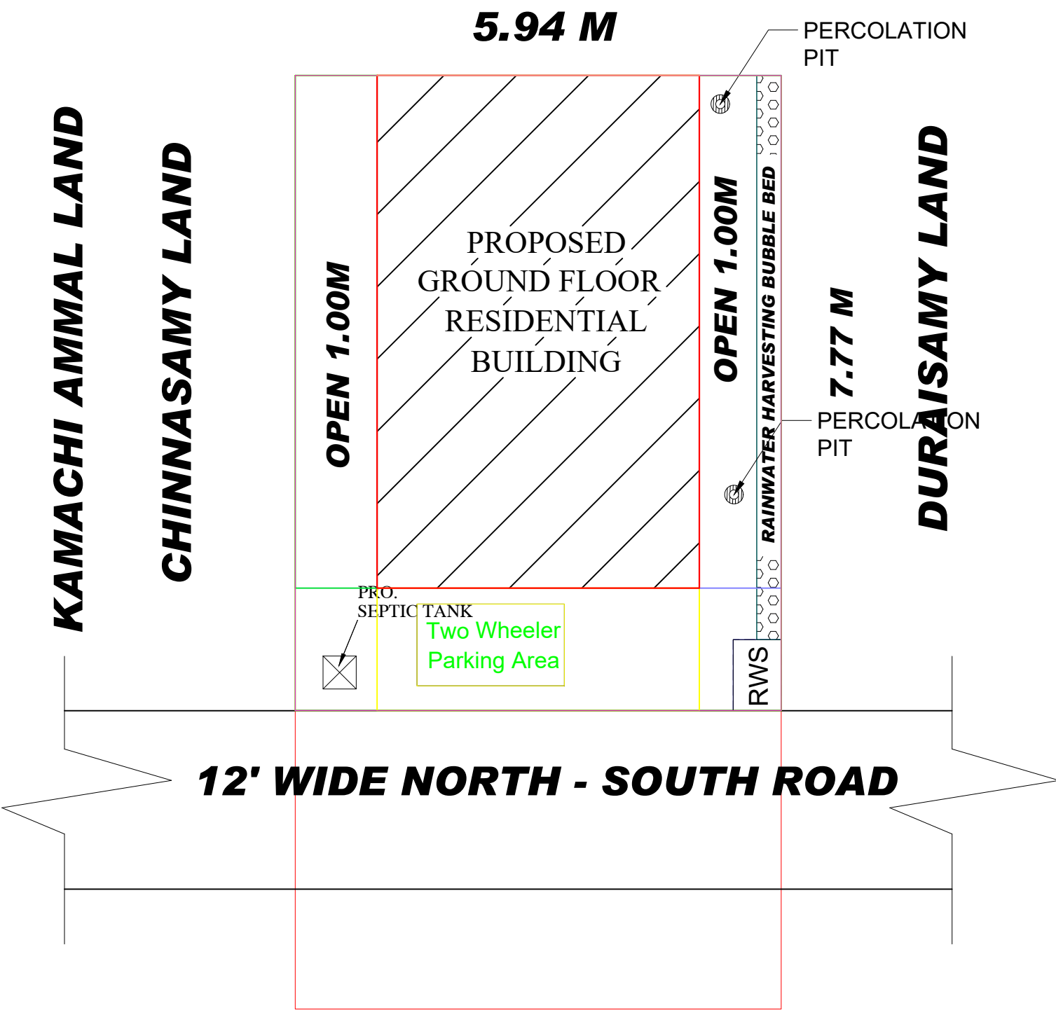
SITE PLAN (SCALE 1:1)
