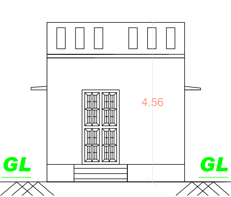
FRONT ELEVATION
