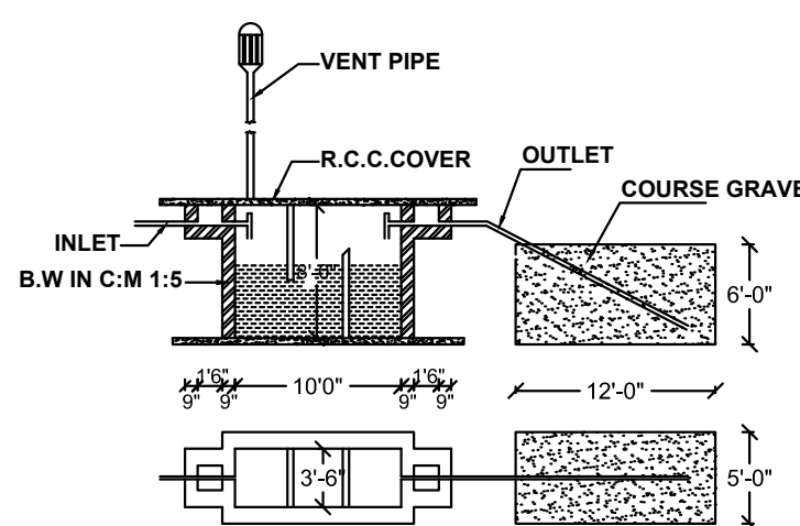
SEPTIC TANK & D-TRENCH DETAILS (NOT TO SCALE)
