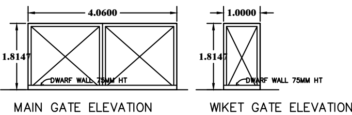
MAIN GATE ELEVATION
