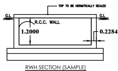
RWH CAPACITY L=2000LTRS
