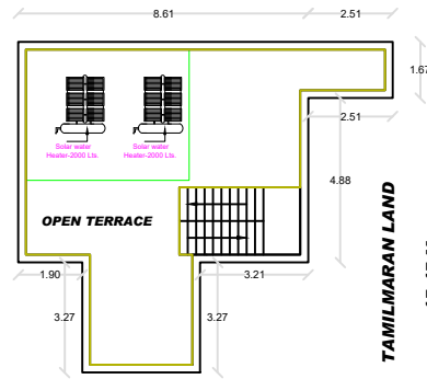
OPEN TERRACE PLAN
