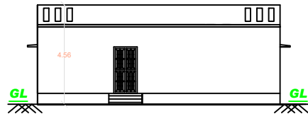
FRONT ELEVATION
