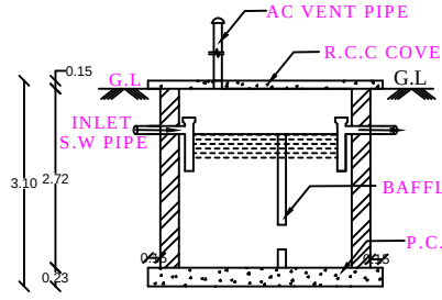
SAEPTIC TANK DETAILS
