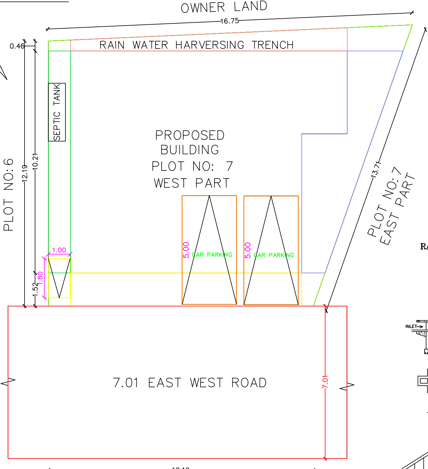
SITE PLAN
