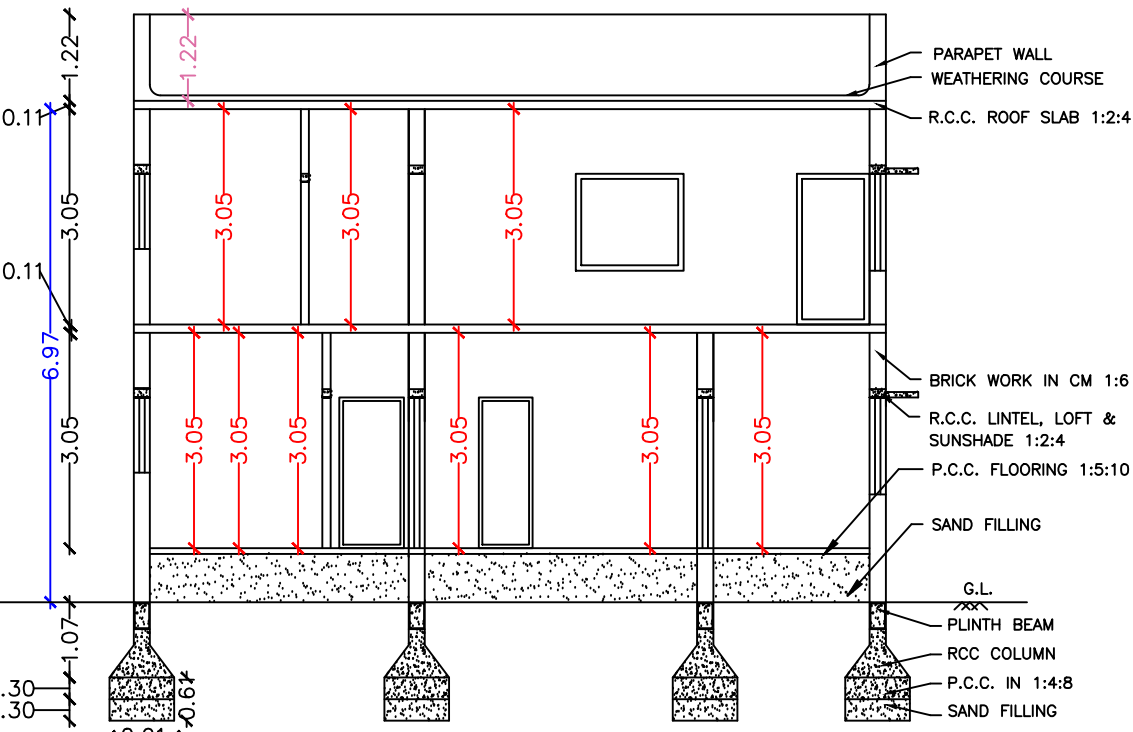
SECTION AA
