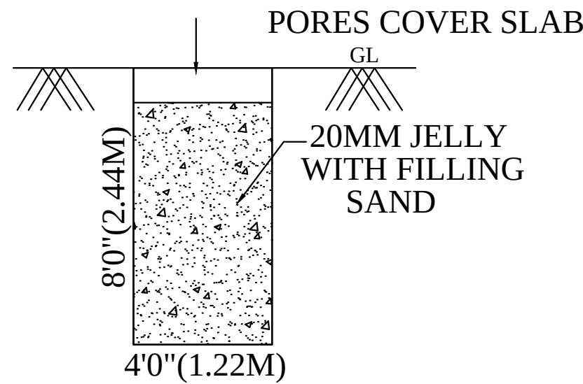
RAINWATER HARVESTING UNIT
