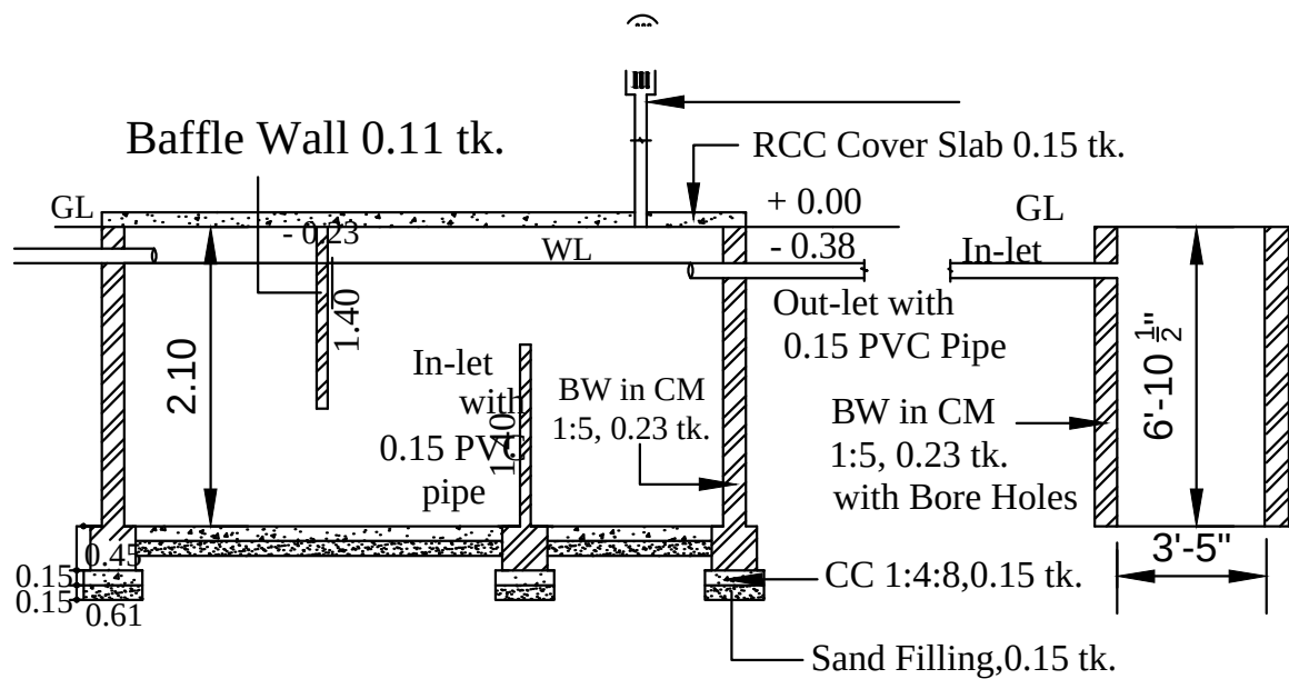
SECTION - SEPTIC TANK & SOAK PIT
