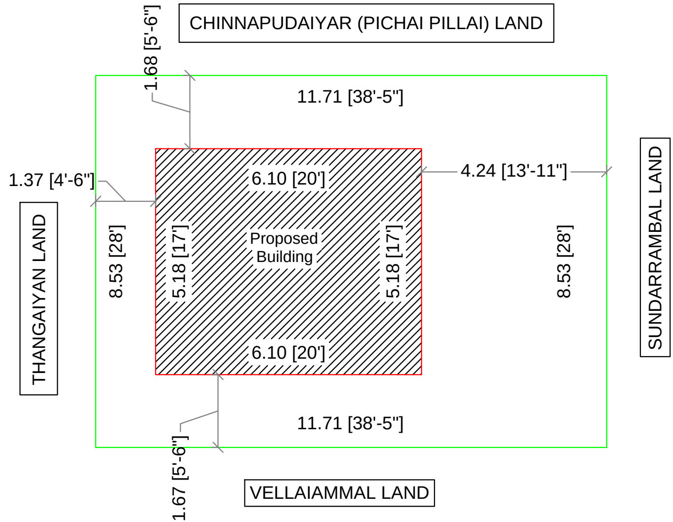
SITE PLAN
