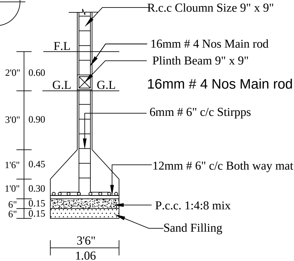
COLUMN DETIAL
