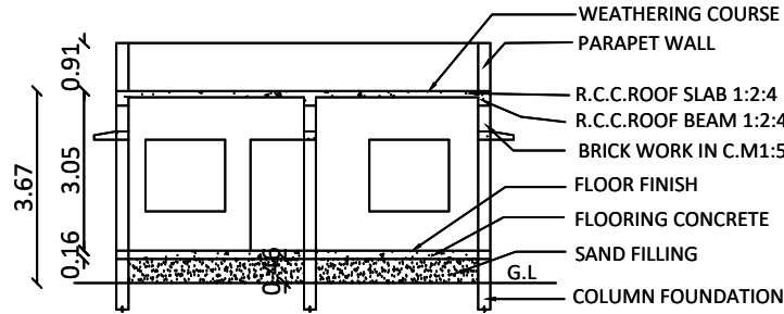
SECTION- SS
