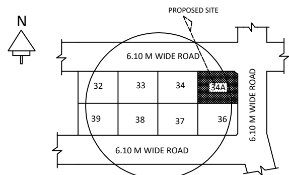
LOCATION PLAN
