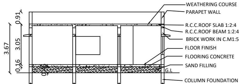
SECTION- SS
