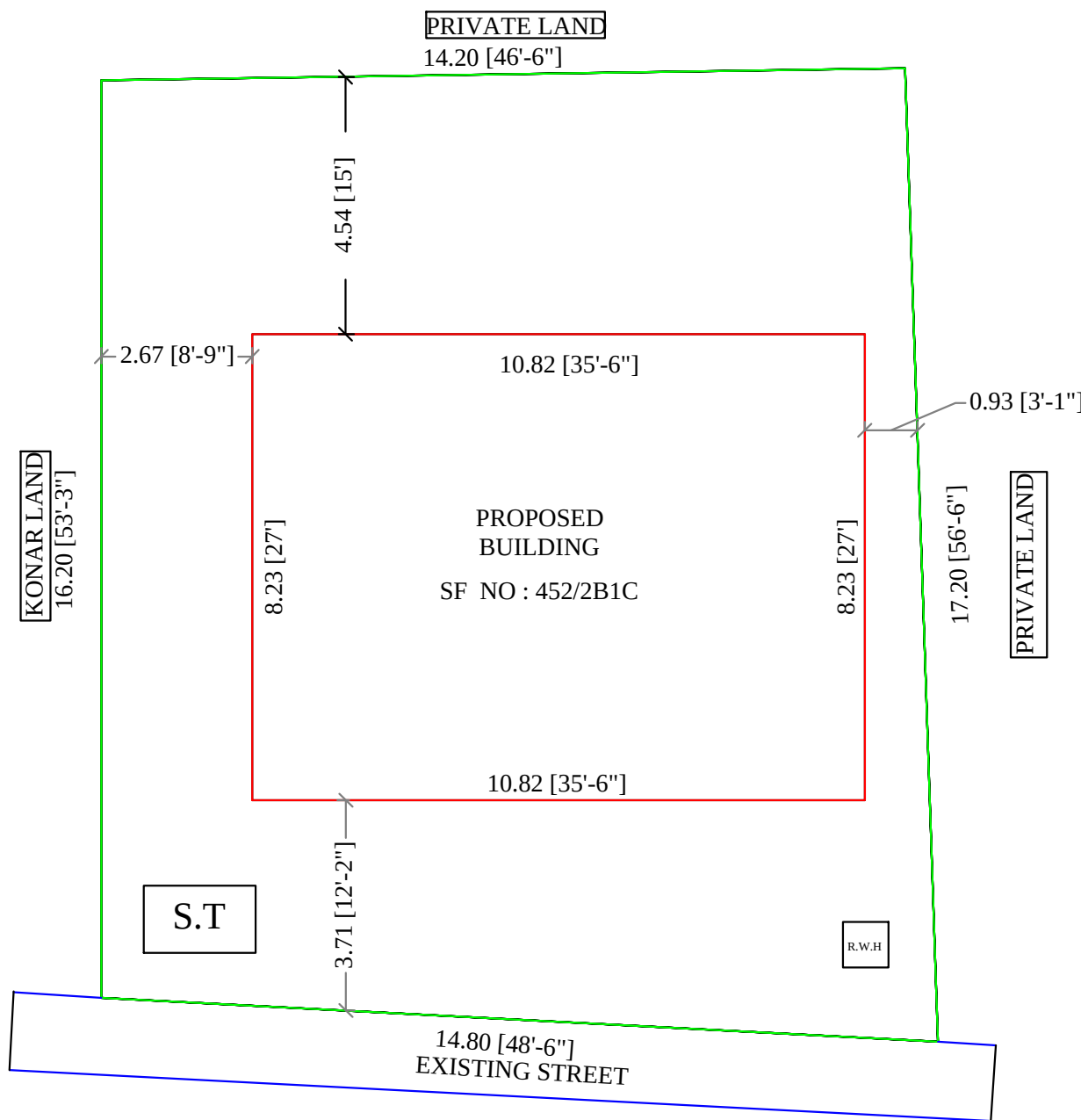
SITE PLAN
