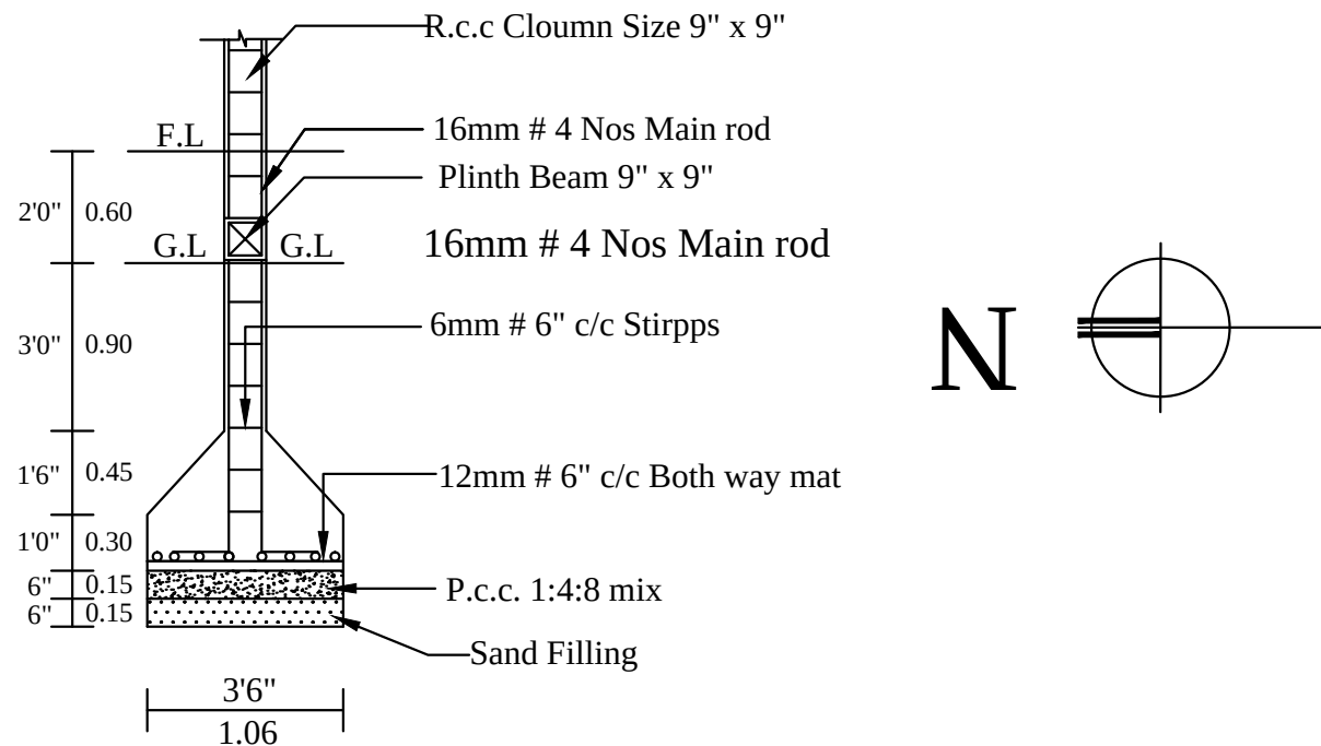
COLUMN DETIAL
