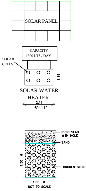
RAIN WATER HARVEST COLLECTION PIT.
